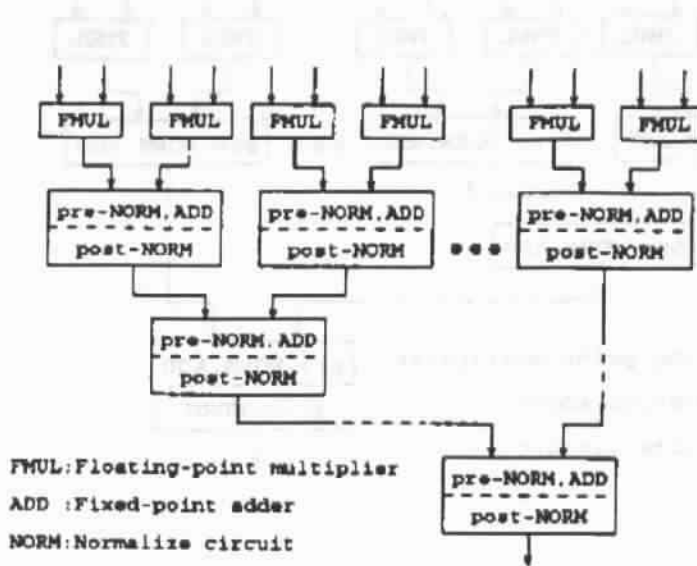
Figure 12: Conventional floating-point multi-operand multiply-adder.
