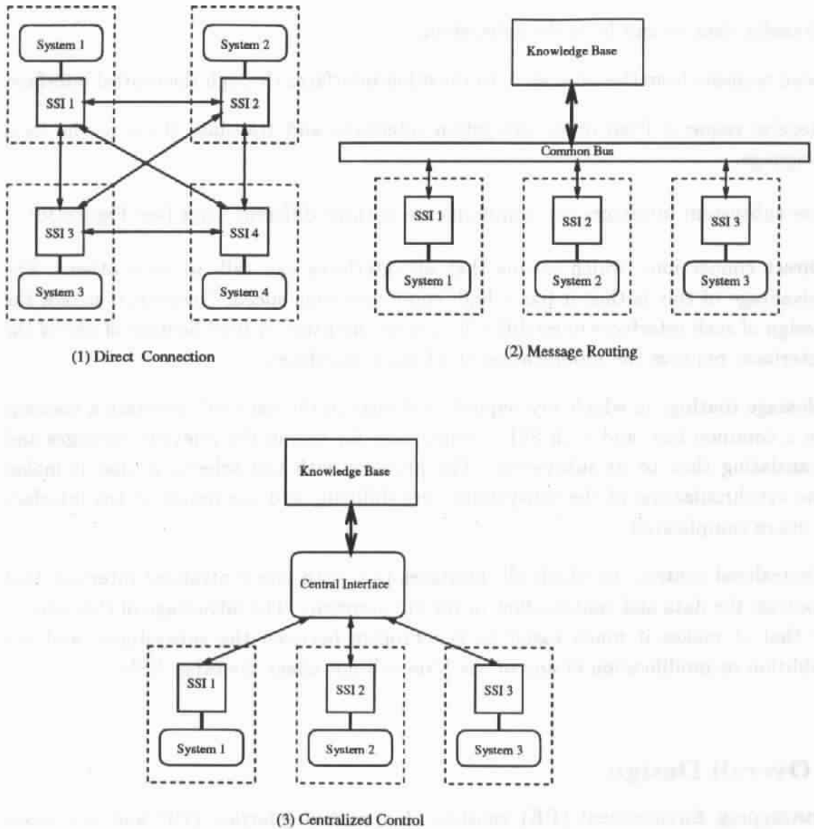
Figure 30: Three different methods for subsystem interface communication.
