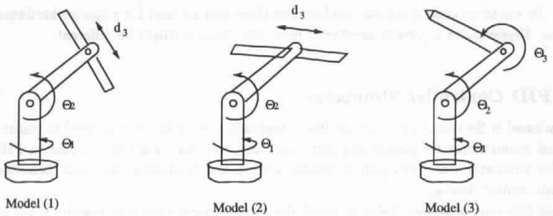
Figure 19: Three different configurations of the robot manipulator.
