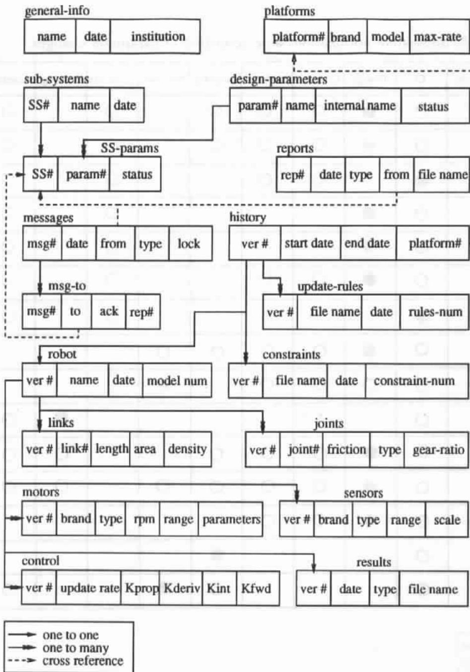
Figure 37: Database design for the system.
