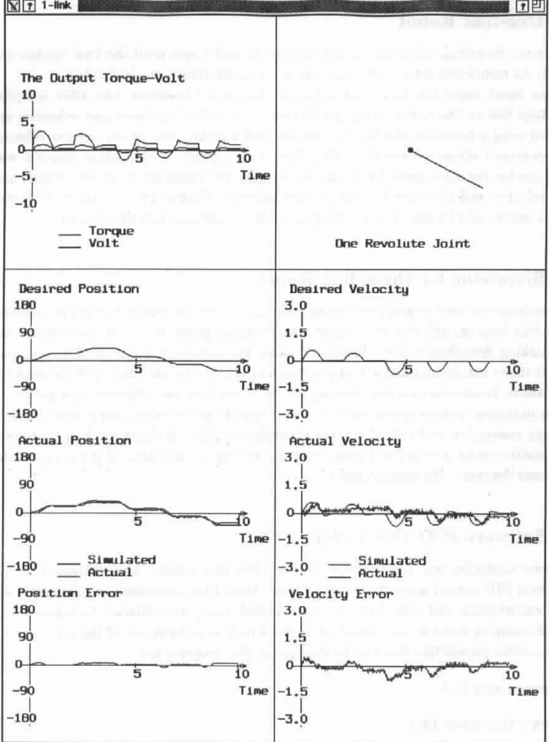
Figure 44: The behavior of the one-link robot for the first input sequence.
