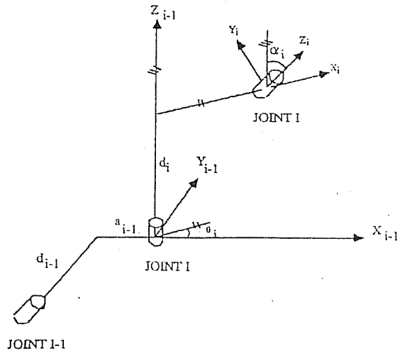
Fig. 1 The relationship between consecutive links.
